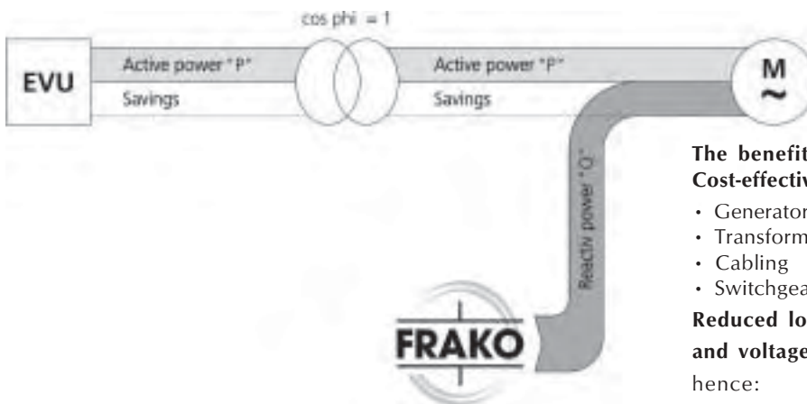
Fig. 7: Active and reactive power in the power distribution system: with correction
