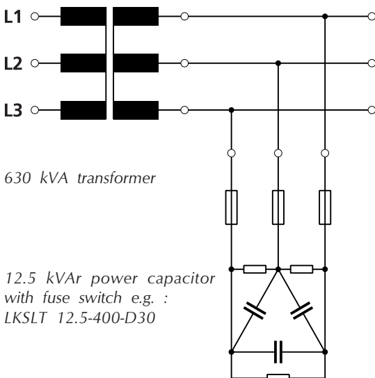
Fig. 16: Typical transformer with permanent power factor correction
