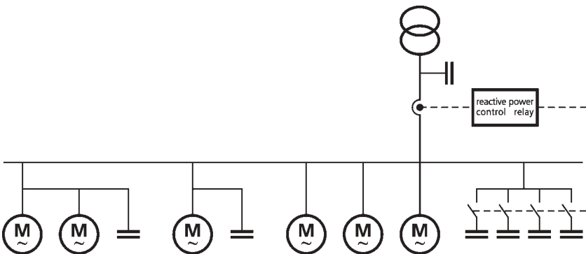
Fig. 11: Typical hybrid power factor correction system
