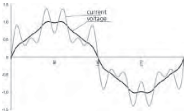
Fig. 30: Network current and voltage superimposed with the following harmonics:
