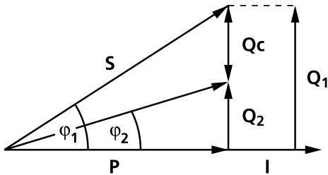
Fig. 5: Power triangle showing the effect of correction
