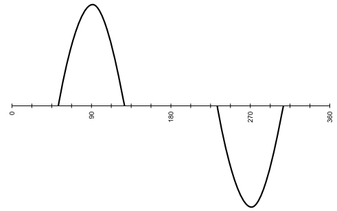
Fig. 32: Current of a power rectifier
