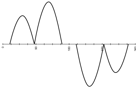
Fig. 31: Mains current of a converter for induction motors
