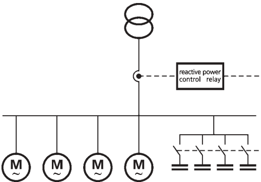
Fig. 10: Typical central power factor correction system
