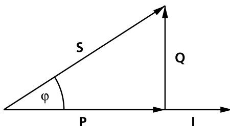
Fig. 4: Power triangle
