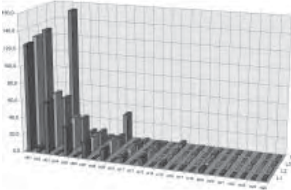
Fig. 44: Harmonics measured, without filter
