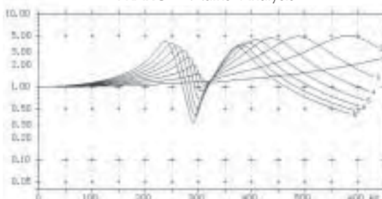
Fig. 39: Amplification of the harmonics when using an unchoked power factor correction system with an AF rejector circuit for 316.7 Hz
