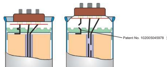
Principle of the overpressure disconnection system
