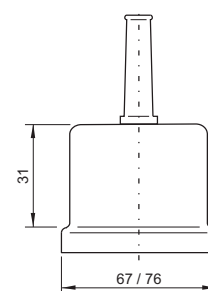
Plastic cap and rubber sleeve LKK 60/70 for capacitors with: d = 60 mm (Art.No. 69-00352) / d = 70 mm (Art.No. 69-00350) (not available for capacitors with d = 85 mm) Rubber sleeve for insulating cap Art.-No. 69-00353
